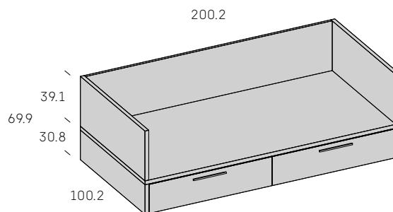
Nido Praktic 2 cajones alto 30.8 cms. Cierre
