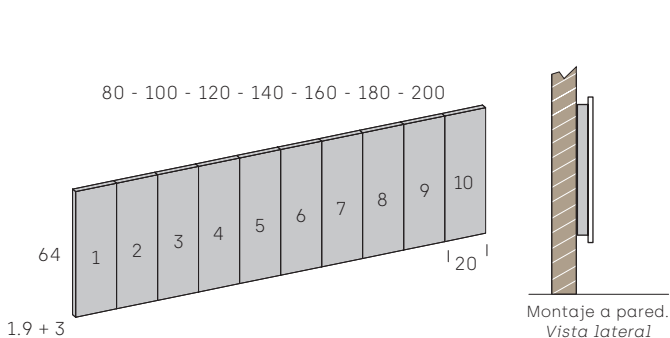
Cabezal Olimpia Light Vertical de 64 cms.
