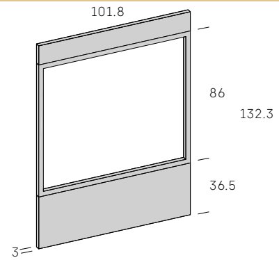
Lateral metal base cama Block
