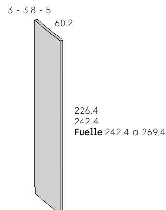
Montante recto lateral 60.2 cms. fondo
