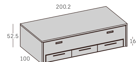
Compacto DUO 2 camas + 3 cajones. Alto Complet 3 cms. grueso
