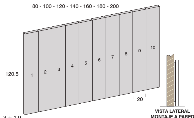
Cabezal Olimpia Vertical de 120.5 cms.
