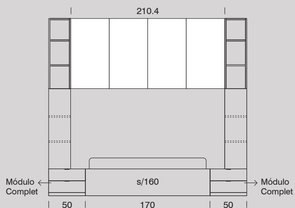
Altillo 210.4
